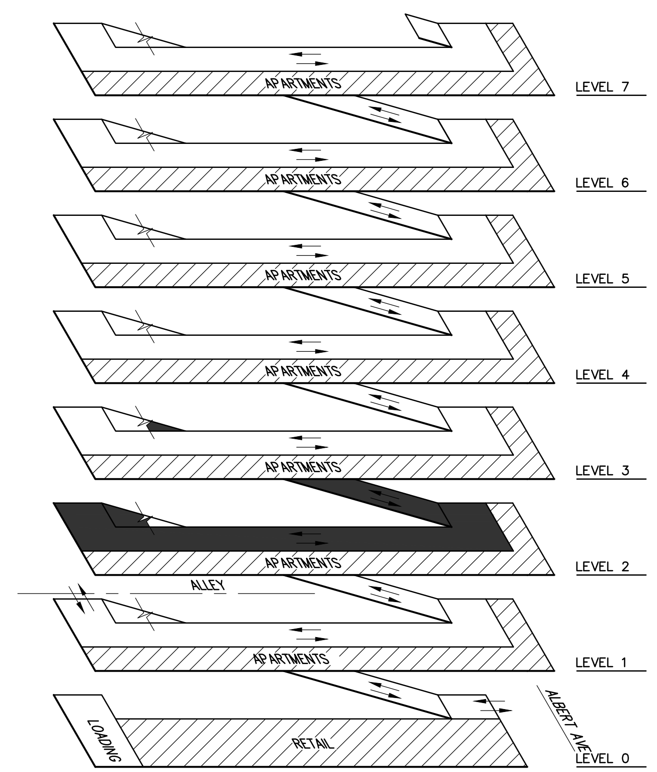
ISOMETRIC NO SCALE X-N1-2013-068-ISO
