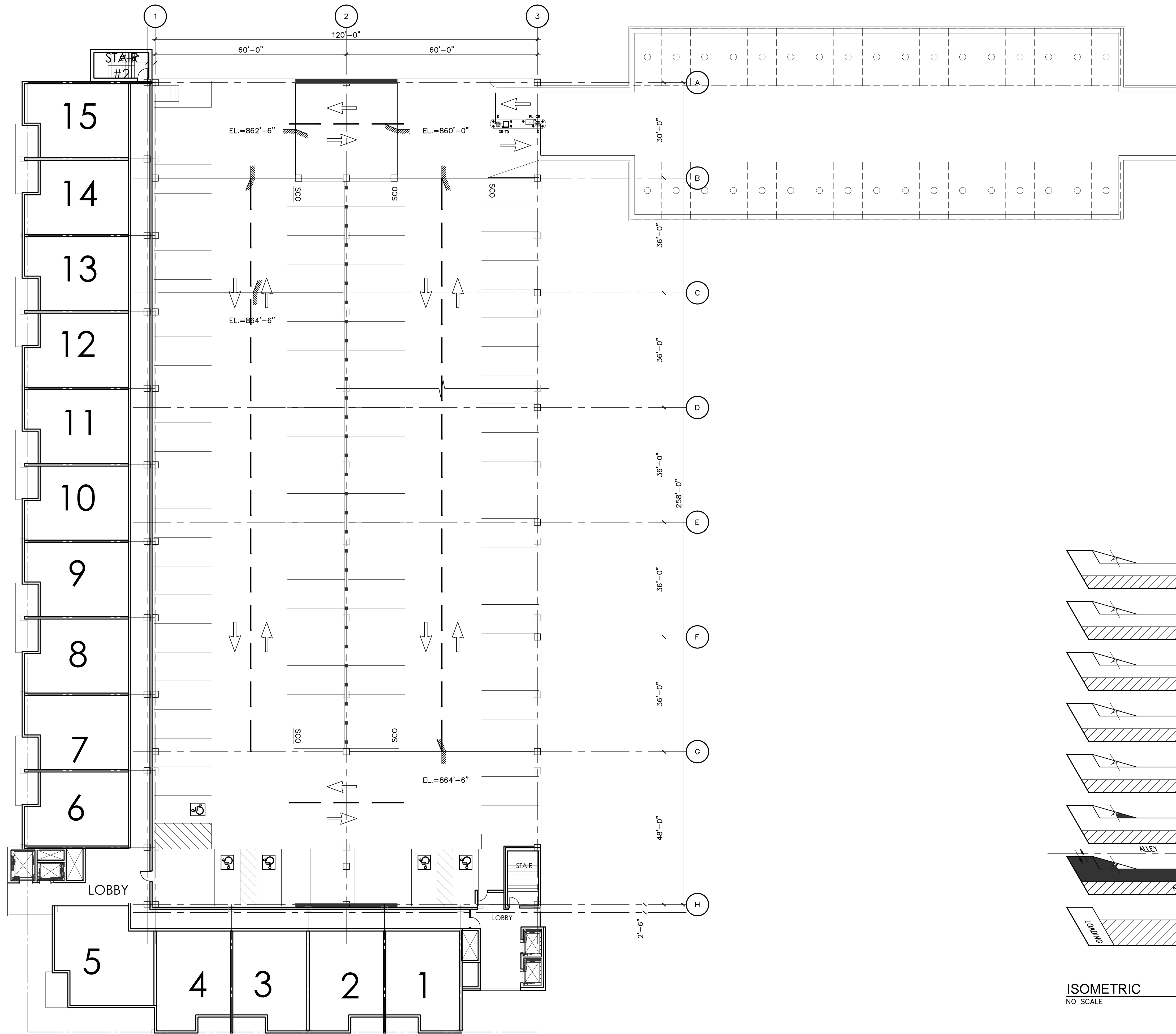
LEVEL 1 FUNCTIONAL PLAN 1/16"=1'-0"
